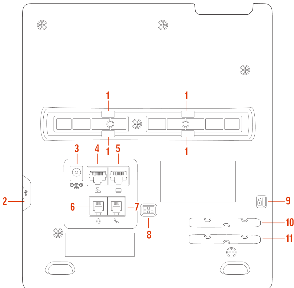
Poly Edge E300 Series phone hardware features - back
